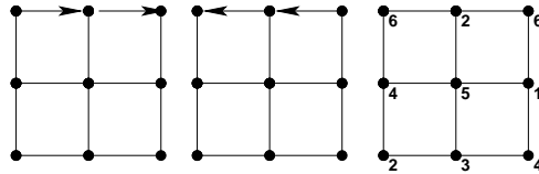
Figure 8: An oriented coloring (right) if the situations depicted (left and middle) do not appear
