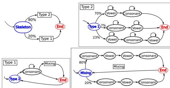
Fig 3: Stochastic Finite State Automata for Consonant Skeleton
