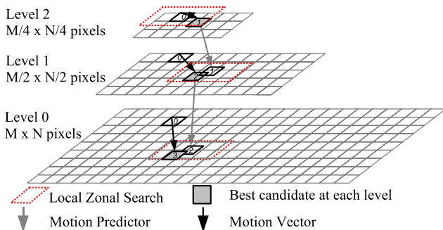
Fig. 2 Pyramid of pictures in HME
