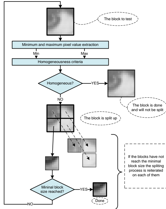
Figure 2: Partitioning Algorithm
