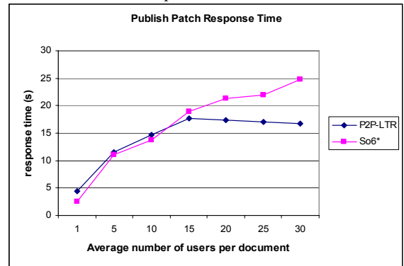
Figure 6. Response time vs. number of users.
