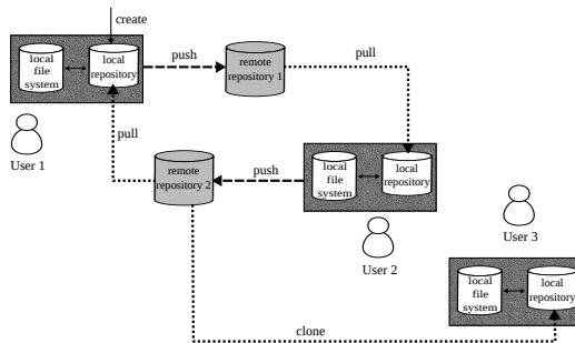
Figure 1: Push-Pull-Clone paradigm
