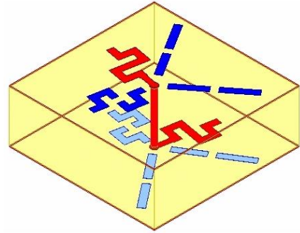
Figure 6. Optimised proposed cell with crank 4 activated
