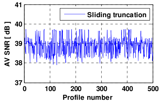
Fig. 20 AG SNR for v = 4 km/h for TGn model B architecture.
