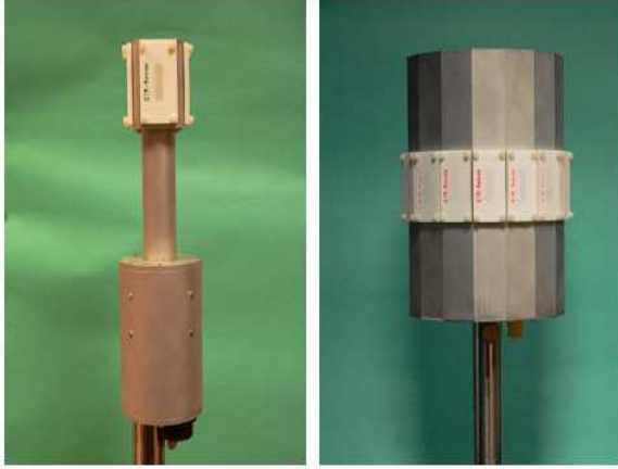
Fig. 5 UCA 4-element transmitter (left) and 16-element receiver (right).
