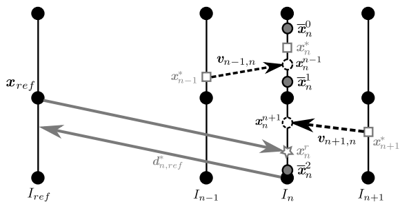
□ previous estimation ● K initial candidates ☆ candidate coming from \mathbf{d}_{n,ref}^* inverted Figure 2: The displacement field \mathbf{d}_{ref,n}^* is questioned by generating for each pixel \mathbf{x}_{ref} competing candidates in I_n .
