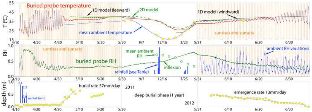
Figure 8. Data from probe 1 buried from April 2011 to July 2012. Top: three panes show buried temperature versus time. Timescales are magnified during burial and emergence phases to illustrate near-surface temperature oscillations similar to those discussed in section 3. Small red circles are individual buried temperature measurements at 1 h intervals; they merge into a thick red line as diurnal fluctuations attenuate. Vertical solid orange and dashed lines mark sunrises and sunsets, respectively. Data from 2 February 2012 to 14 April 2012 are interpolated from adjacent records when memory overflowed. The dashed blue line is the periodic fit (equation (C1)) of monthly averaged ambient temperatures measured on our weather station (circles) for 12 months prior to November 2011. (Triangles are extrapolations from 2012 values for temperatures unrecorded prior to weather station setup). The dashed black line is the 1-D thermal model of equation (D7). The dashed green line is from the 2-D model in Figure 7. Middle: three panes show RH (or water activity, green line), with inflexion around 17 December. Vertical blue lines are proportional to rainfall quoted in Table 1. The blue line and green circles are, respectively, instantaneous and monthly averaged relative humidity. Bottom: two panes separated by a whole year show daily burial depth inferred from peak temperature time lags after solar noon.
