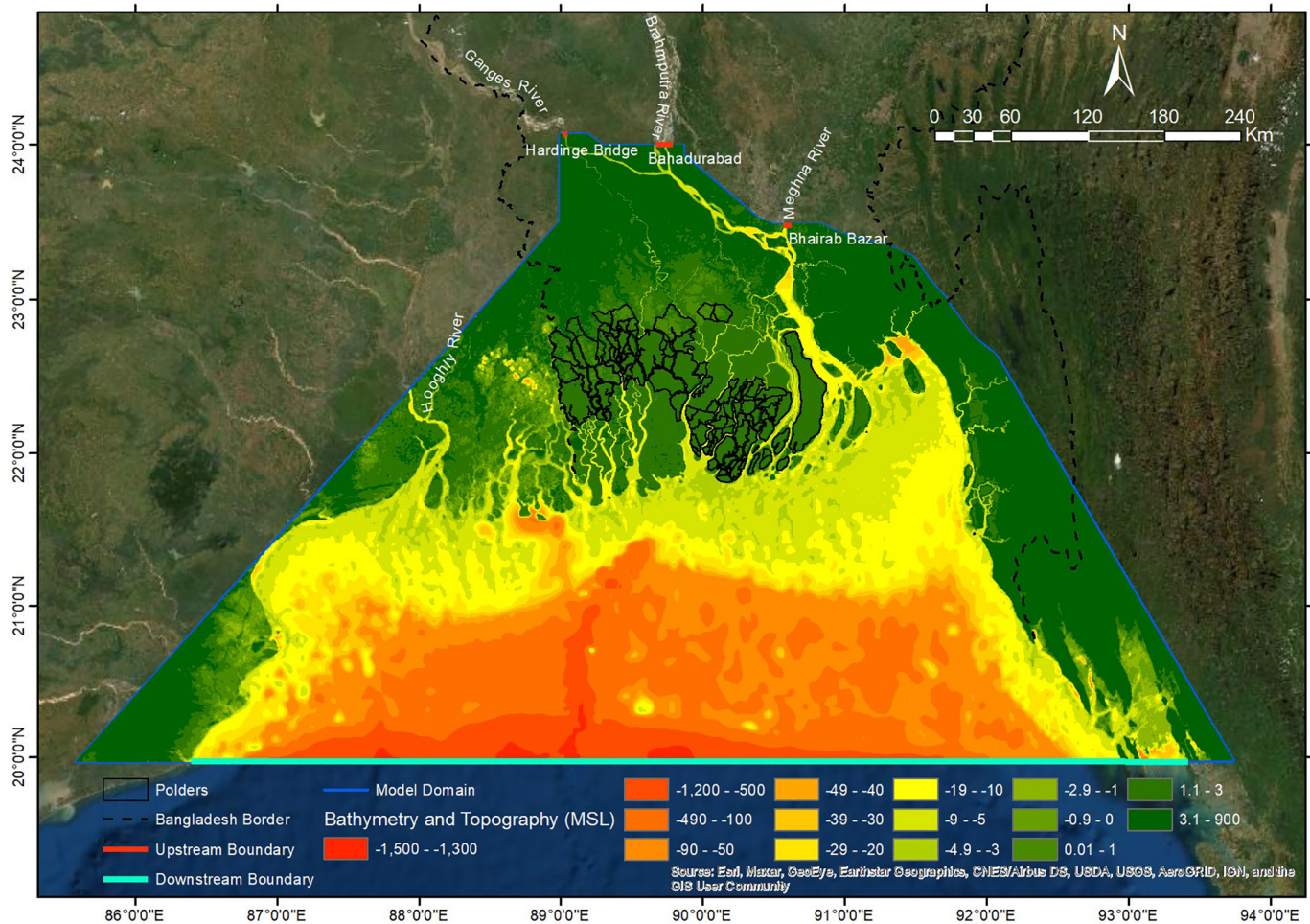
Fig. 2. The model domain, including the major rivers, topography and bathymetry. The topography and bathymetry are measured in meters from Mean Sea Level (MSL). The model domain covers the coastal part of the Ganges-Brahmaputra-Meghna delta, and the Bangladesh territory is shown by black dotted lines. Locations of the three upstream river discharge boundaries and the downstream sea level boundaries are marked. The black firm lines represent the polders.
