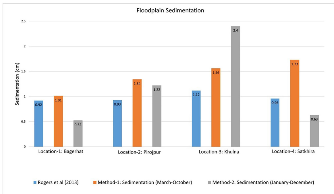
Fig. 3. Comparison of floodplain sedimentation in the Sundarban region between modelled and measured data (Source of measured data: Rogers et al., 2013). All the measurement locations are in Sundarban region (see Fig. 1). Location-1 is in Bagerhat district, location-2 is in Pirojpur district, location-3 is in Khulna district, and location-4 is in Satkhira district. Method-1 shows the sedimentation for 8 months model simulation (March–October) whereas, Method-2 shows the sedimentation for 12 months model simulation (January–December). Both the measurement and the model simulations are for the year 2008.
