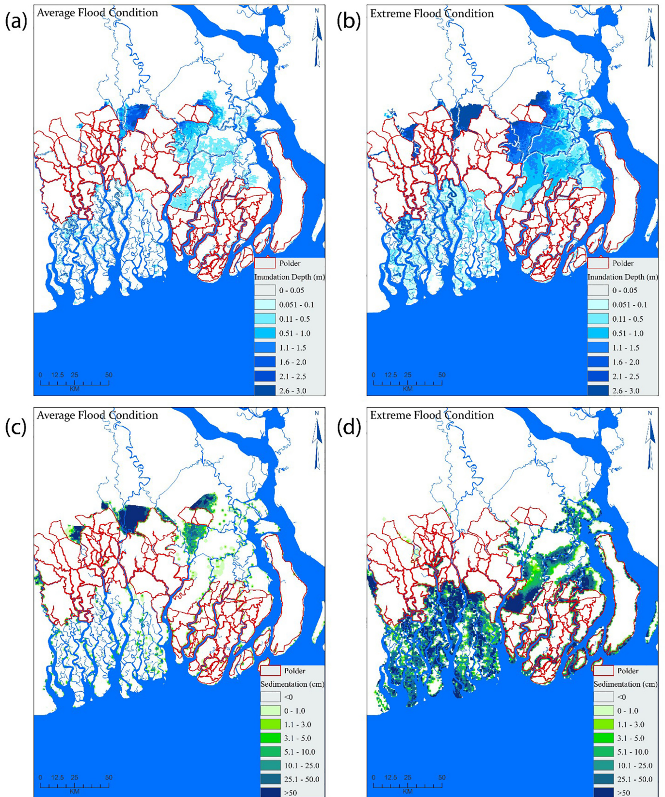
Fig. 4. Maximum inundation (a and b) and annual sedimentation (c and d) in the intervened delta state during average flood and extreme flood conditions, respectively. The red lines show the polder embankments. Only part of the unprotected land is inundated during average flood condition (a). The extent and severity of inundation increases with the intensity of flooding (b). Sedimentation occurs in the areas which are flooded (c and d). Following the inundation patterns, sedimentation only occurs on part of the inundated land (c) and increases with the depth and area of inundation (d).
