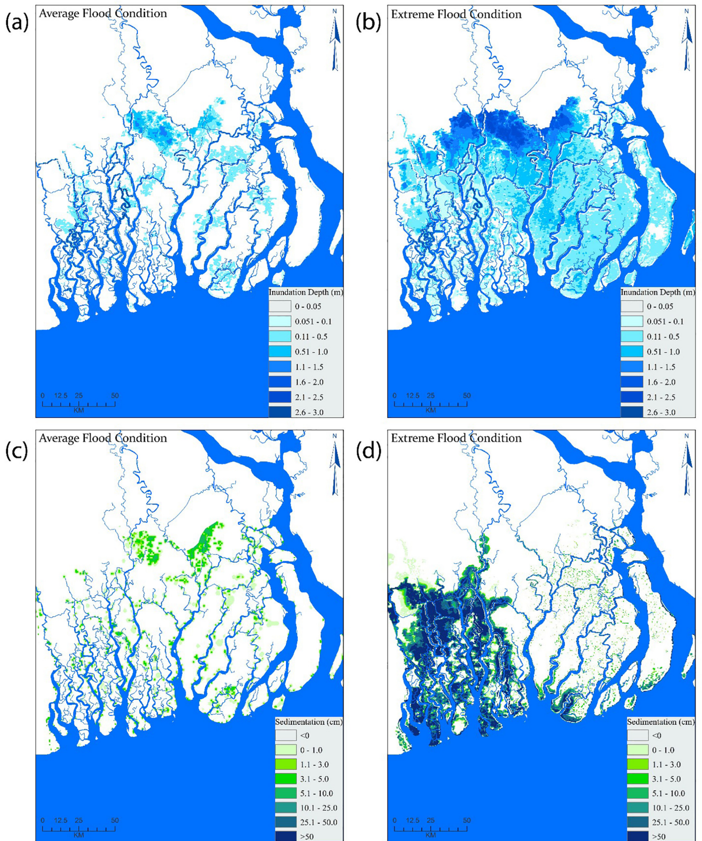
Fig. 5. Maximum inundation (a and b) and annual sedimentation (c and d) in the natural delta state for average flood and extreme flood conditions. The inundation of the delta in the natural state depends entirely on the flooding condition, existing river and canal bathymetry, and land topography: less inundation during an average flood condition (a) as compared to an extreme flood condition (b). For average flood conditions, sedimentation occurs in the delta region where inundation depth is relatively high (c). For extreme flood conditions, higher flow resistance in the Sundarban region increases sedimentation (d).
