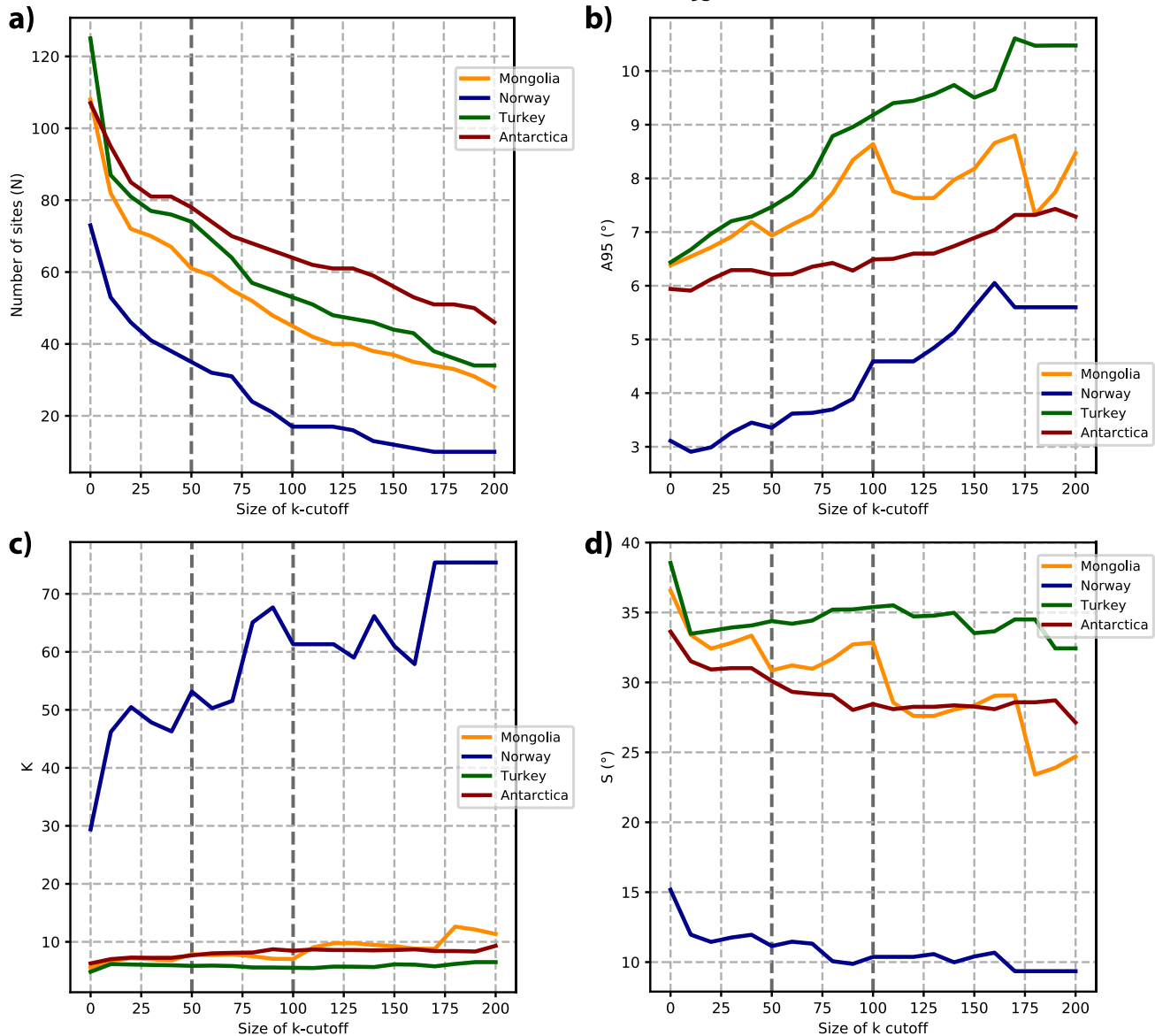
Figure 4. Effect of the size of the k -cutoff on (a) the number of sites ( N ) remaining in the data set after application of the cutoff, and the (b) A_{95} , (c) K , and (d) S of the acquired paleopole. Commonly applied cutoff sizes of 50 and 100 are indicated with gray dashed lines.
