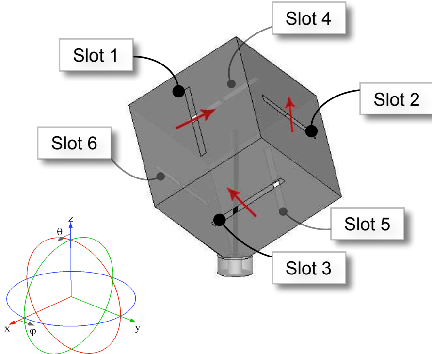
Fig. 1 - Schematic drawing for the reconfigurable cubic antenna
