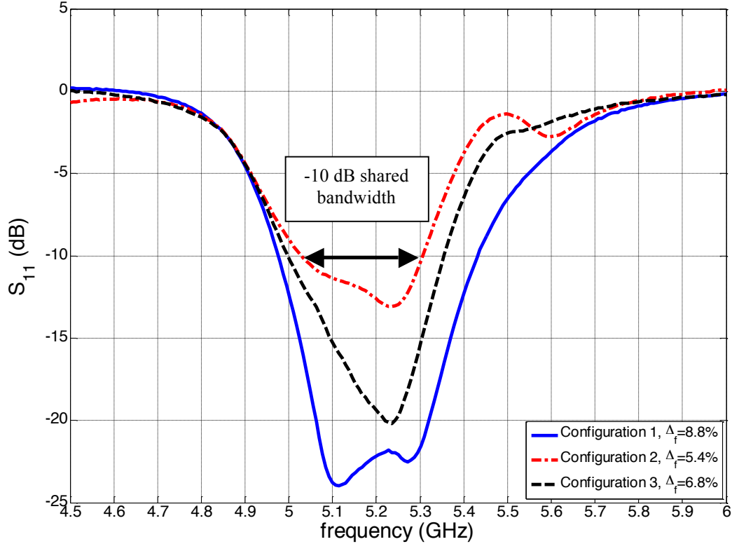
Fig. 11 - Reflection coefficient of the build antenna in the three pattern configurations
