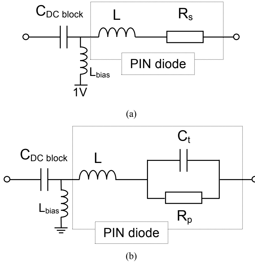
Fig. 7 – RF equivalent circuit for PIN diode and DC block capacitance in the (a) ON state (forward bias) and (b) OFF state (reverse bias)
