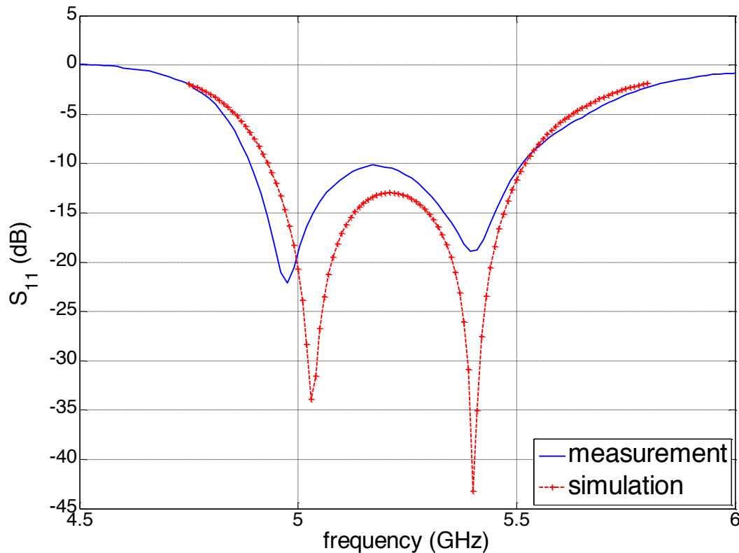
Fig. 3 - Comparison of simulated and measured reflection coefficient for the dual-resonance antenna
