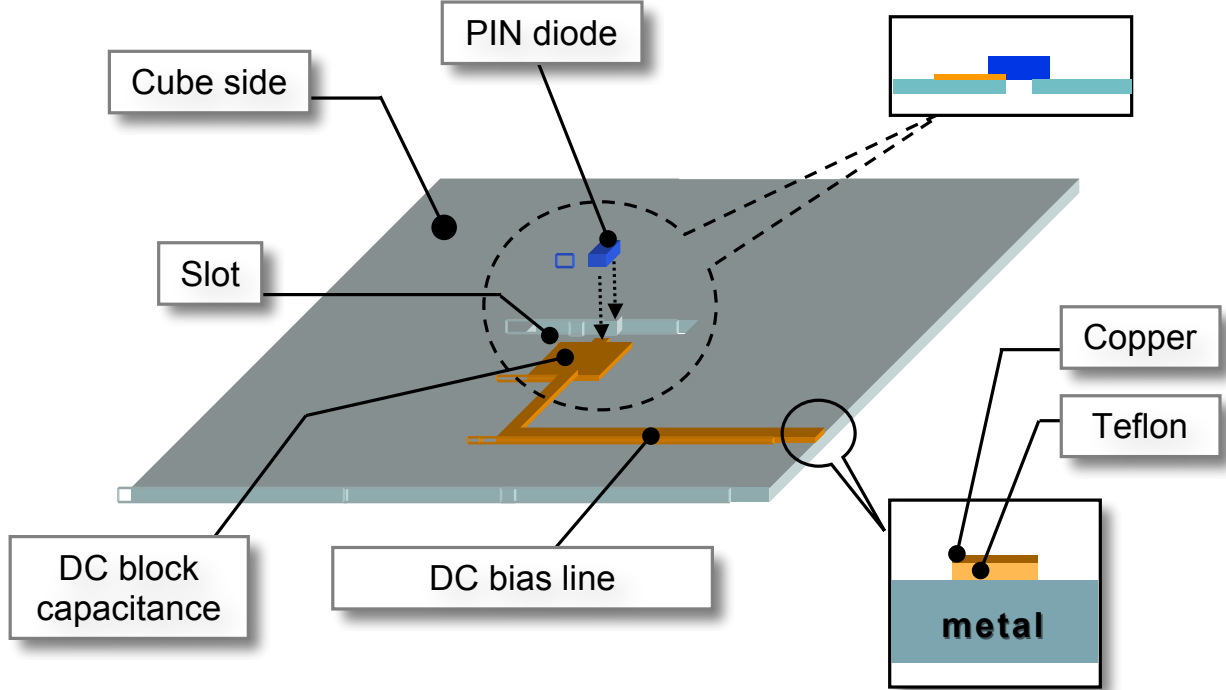
Fig. 6 - PIN diode location on a cube side with DC bias circuit
