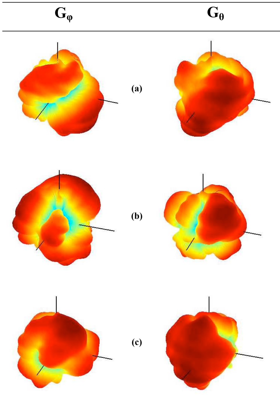
Fig. 12 - Measured radiation patterns along \varphi (on left) and \theta (on right) for (a) configuration 1, (b) configuration 2 and (c) configuration 3
