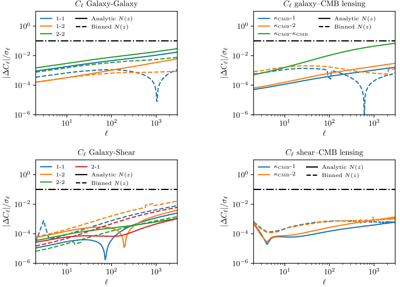
Figure 13. Same as Figure 12 for angular power spectra involving CMB lensing. The black dot-dashed line indicates the target numerical accuracy of 0.1\sigma_\ell . Top : cross-correlations with number counts and CMB auto-correlation. Bottom : cross-correlations with weak lensing.
