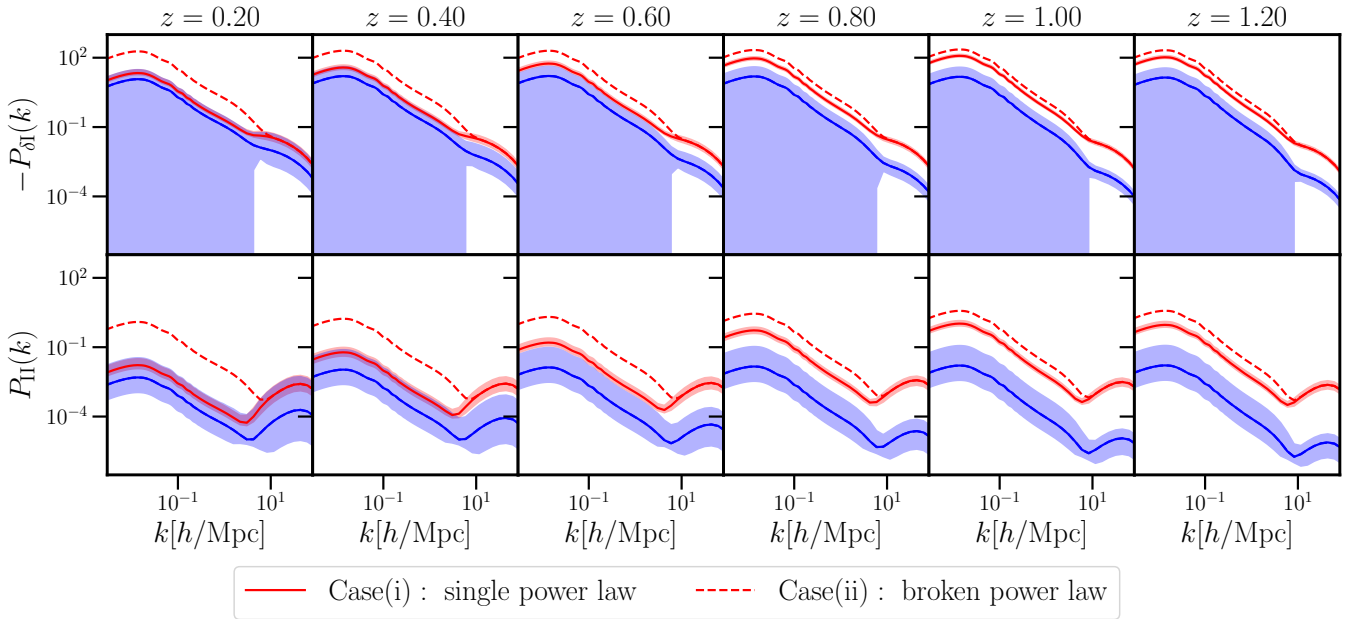
Figure 8. The matter - intrinsic and the intrinsic-intrinsic shear power spectra for our case (i) (solid lines) and (ii) (dashed lines). The red curve corresponds to the red sample, the blue curve to the blue sample. The shaded areas corresponds to the 1\sigma uncertainties in the model as derived from the parameters uncertainties in Tab. (3). For clarity, we only show it for our case (i). For the matter-intrinsic power spectra, we only plot the negative part.
