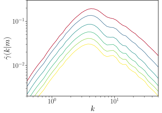
Figure C1. The Fourier transform of the density-weighted shear (eq. 13) for \phi_k = 0 and \theta_k \in [\frac{\pi}{2}, \pi] , in the case of constant radial dependence. For clarity, we normalise the curves by the input amplitude, a_{1h} . The amplitude of the curves decreases as we go from \theta_k = \frac{\pi}{2} (red) to \theta_k = \pi . Note that f(\theta_k) is symmetric around \theta_k = \pi/2 , so the curves from [0, \frac{\pi}{2}] coincide with the ones plotted here, with increasing amplitude for increasing values of \theta_k .
