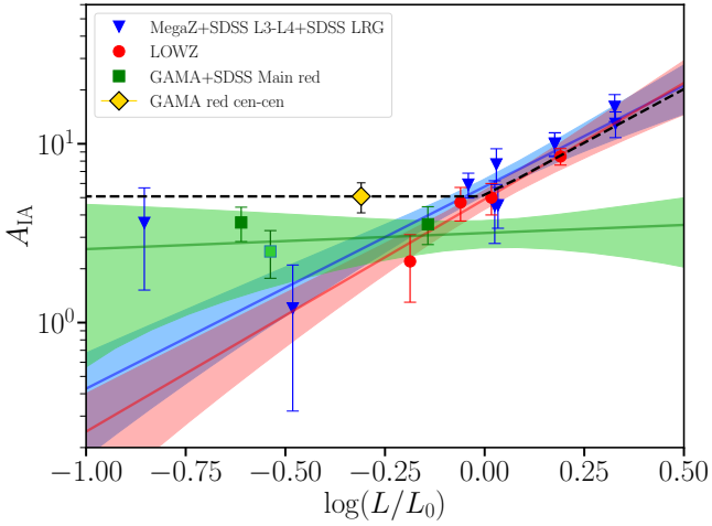
Figure 5. Overview of different estimates of the IA amplitude as a function of luminosity. The best-fit relation from Joachimi et al. (2011) (blue line) for the MegaZ, SDSS L3 and L4 and SDSS LRG samples (blue downward facing triangles); Singh et al. (2015) best-fit (red line) on LOWZ (red circles) and the revised best-fit to GAMA+SDSS Main from J19 reported in the text (green line). The three individual samples used by J19 are shown as green squares (GAMA) and limegreen (SDSS Main sample). The yellow diamond indicates our best fit amplitude for the GAMA red central galaxies.
