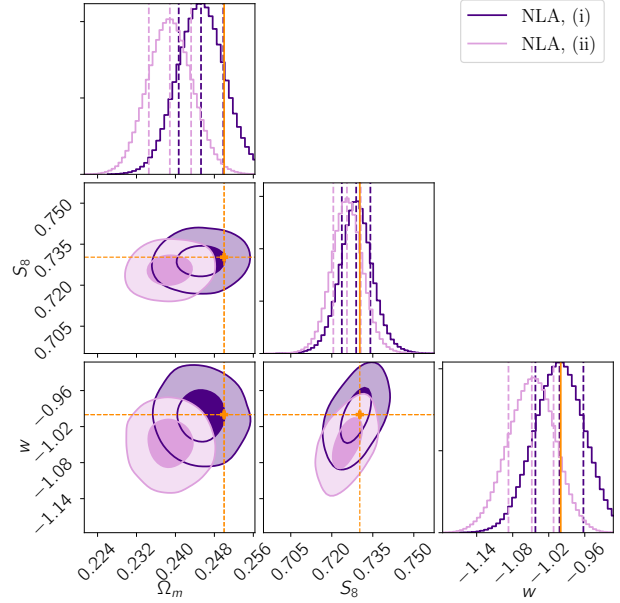
Figure 10. Constraints on the cosmological parameters \Omega_m , S_8 = \sigma_8 \sqrt{\Omega_m}/0.3 and w , marginalising over the IA amplitude, for a Stage-IV survey. We inject the IA signal as predicted by the full halo model formalism assuming at larger scales a steep luminosity dependence (i: indigo) or a broken power law with constant amplitude for faint galaxies (ii: plum) - Table 3 lists the IA parameters used for constructing the data vectors. We perform the analysis assuming a NLA model with no distinction between red and blue galaxies. The orange lines and the square markers indicate the fiducial values of the cosmological parameters.
