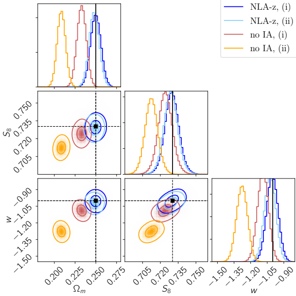
Figure 11. Constraints on the cosmological parameters \Omega_m , S_8 = \sigma_8 \sqrt{\Omega_m}/0.3 and w , marginalising over the IA amplitude, for a Stage-IV survey. We distinguish between two IA scenarios at large scales, as detailed in Table 3. We perform the analysis assuming no distinction between red and blue galaxies and assume either a NLA- z model (dark blue ellipse for the IA signal as in case (i) and light blue ellipse for the case (ii)) or no IA (red for the IA signal based on (i), orange for the (ii)). The black lines and the square markers indicate the fiducial values of the cosmological parameters.
