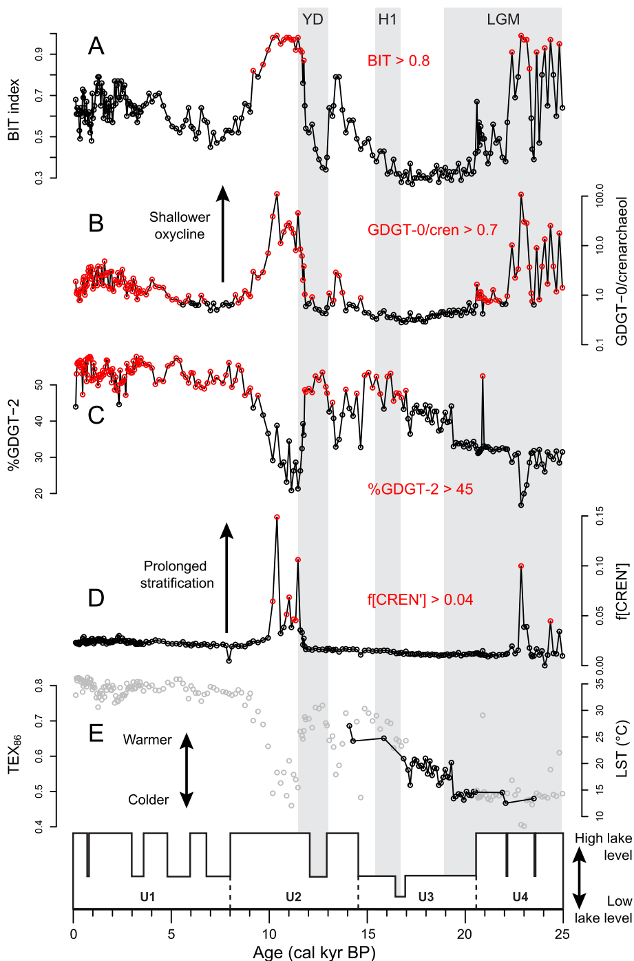
Fig. 8. Temporal variation in BIT index (A; from Verschuren et al., 2009); (B) GDGT-0/crenarchaeol ratio (B); %GDGT-2 (C), f[CREN'] (D) and TEX 86 (E; the latter all modified after Sinninghe Damsté et al., 2012a) in the 25-kyr sediment record of Lake Chala, compared with the succession of lake high- and low-stands based on seismic-reflection stratigraphy (F; from Moernaut et al., 2010). In panels A–D, GDGT proxy values outside the boundaries proposed for reliable TEX 86 -based temperature reconstruction are indicated in red; see text. In panel E, reliable TEX 86 datapoints are plotted in black, while compromised values are plotted in light grey. The shaded areas represent the Last Glacial Maximum (LGM; 23–19 ka BP), Heinrich event H1 (16.8–15.4 ka BP) and the Younger Dryas period (YD: 13–11.5 ka BP). (For interpretation of the references to color in this figure legend, the reader is referred to the Web version of this article.)
