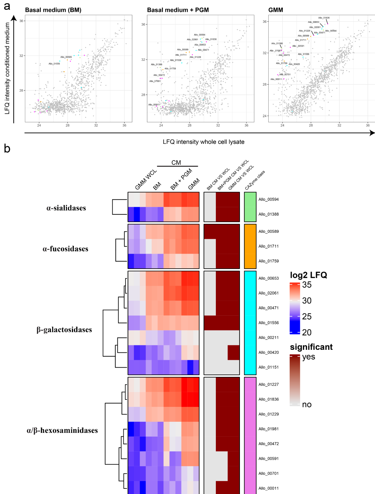
Figure 3. Mass spectrometry analysis of the A. mucolyticum proteome demonstrates the presence of mucin O -glycan targeting CAZymes. Conditioned media (CM) from 24 h cultures in basal medium (BM), basal medium + PGM and Gut Microbiota Medium (GMM) and a whole cell lysate (WCL) from the GMM culture were subjected to mass spectrometry analysis, with three biologically independent replicates per condition. (a) The scatter plots show the log 2 LFIQ from whole cell lysate of the GMM culture (X-axis) and the secretomes from the three different media (Y-axis). The colored dots indicate the putative O -glycan targeting CAZymes with their color matching the color of their putative CAZyme class shown in the heat map. (b) The red/blue heat map displays the proteins and their relative enrichment in the three different secretomes compared to the GMM WCL. Significance (depicted in the brown heatmap) was calculated using a t-test and indicates a > 10 fold enrichment in the respective secretome versus GMM WCL with an FDR < 0.05.
