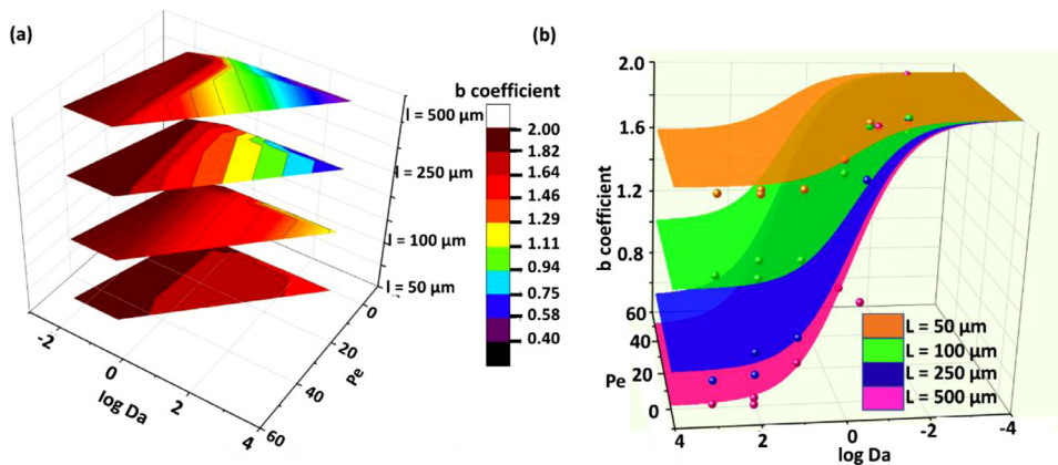
Fig. 6. pore conductance parameters. (a) Dependency of the b coefficient (shown using the color legend) on the strength of reaction and flow regime (the horizontal axes) and pore throat lengths (shown as segregated colors. i.e., each surface corresponds to a certain pore throat length). Higher values of b coefficient correspond to higher Pe numbers and lower Da numbers. Pore throat length of value of 500.0 \times 10^{-6} m shows a higher range for the b coefficient compared to a smaller pore throat length with a value of 250.0 \times 10^{-6} m. (b) the fitted curved surface together with the data points used to obtain the best fit (SI Section S1; Table S1).
