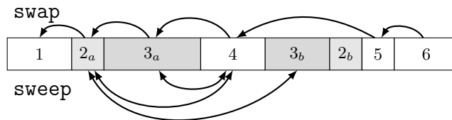
Fig. 1: Overloading decisionList(D) for the relaxation 1|r_j; \text{prec}; \text{pmtn}|L_{max} .
