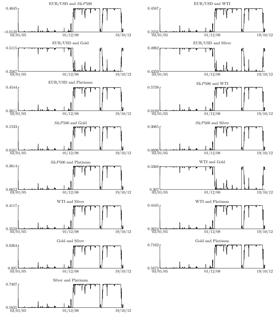
Figure 4: Estimated correlations.
