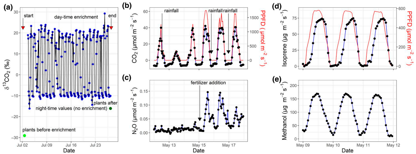
FIGURE 3 Examples of ecotron isotopic labelling and process measurements: Air 13 CO 2 enrichment and plant 13 C labelling in one macrocosm of the Montpellier Ecotron (a); measurements of net ecosystem CO 2 exchange (b) and net ecosystem N 2 O exchange (c) with photosynthetic photon flux density (PPFD) in one macrocosm of the same ecotron; measurements of the emission of two volatile organic compounds (isoprene and methanol) with PPFD in one of the sub-chambers of the München ExpoSCREEN facility (d, e)
