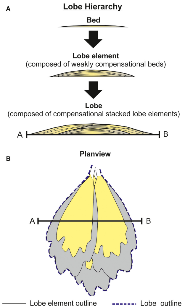
Fig. 11. (A) Diagram of lobe hierarchy dependent compensation. (B) Planview relationship between lobe elements forming a lobe. Yellow colours mark sand-prone deposits, grey colours mark silt-prone deposits (modified from Straub & Pyles, 2012).
