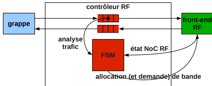
FIGURE 4 – RF controller
