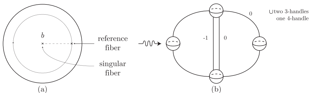
FIGURE 1. Figure (a) shows the base of a boundary Lefschetz fibration over the disc with a single nodal fiber, a choice of regular fiber for reference and loop around the boundary used to compute the monodromy and (b) shows the corresponding Kirby diagram.
