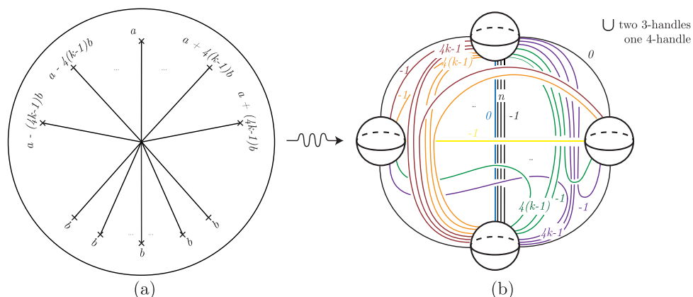
FIGURE 2 (colour online). Figure (a) shows the base of a boundary Lefschetz fibration over the disc with m + n singular fibers and a choice of regular fiber for reference at the center of disc. Figure (b) shows the corresponding Kirby diagram.
