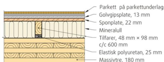
Figur 14 Oppbygning himling. [13]
