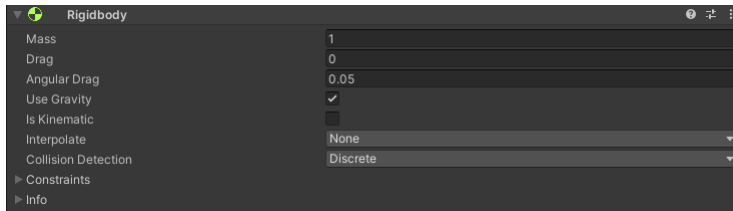
Figure 2.10: Rigidbody Component
