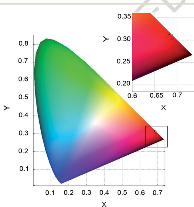
Fig. 4 Representation of [(n\text{-C}_4\text{H}_9)_4\text{N}]_2\text{Mo}_6\text{Br}_{14} (green), PM10 (black circle) and PM50 (blue) ( x ; y ) coordinates in the CIE chromaticity diagram at 293 K for \lambda_{\text{exc}} = 425 nm.
