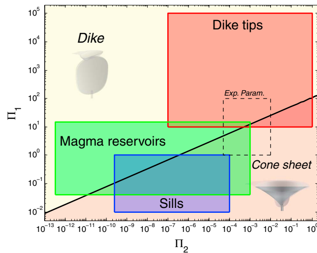
Figure 6. Graph comparing the experimental results of this study (dashed box) to characteristic geological values of \Pi_1 and \Pi_2 . The dike-to-cone sheet transition is extrapolated from the phase diagram of Figure 5. Geological boxes correspond to dike tips (red), magma reservoirs in volcanoes (green), and shallow sills in sedimentary basins (blue). See Table 1 for natural values of \Pi_1 and \Pi_2 .
