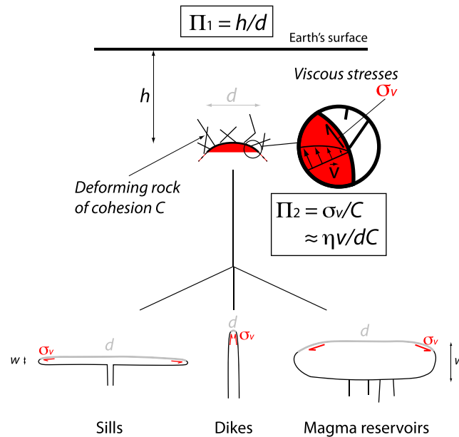
Figure 3. Schematic drawing describing the definitions and illustrating the physical meanings of the main dimensionless parameters \Pi_1 = h/d and \Pi_2 = \eta v/dC used in this study.
