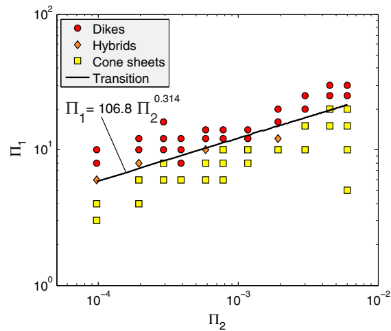
Figure 5. Log-log dimensionless phase diagram distinguishing the intrusion shapes obtained in the 51 experiments of this study: dikes (red circles), hybrid intrusions (orange diamonds), and cone sheets (yellow squares). The axes of the diagram give the initial and boundary conditions expressed by the dimensionless parameters \Pi_1 = h/d and \Pi_2 = v\eta/Cd . The dikes and cone sheet experiments plot in two distinct fields, separated by a line that is defined by the power law \Pi_1 = 106.8 \times \Pi_2^{0.314} .
