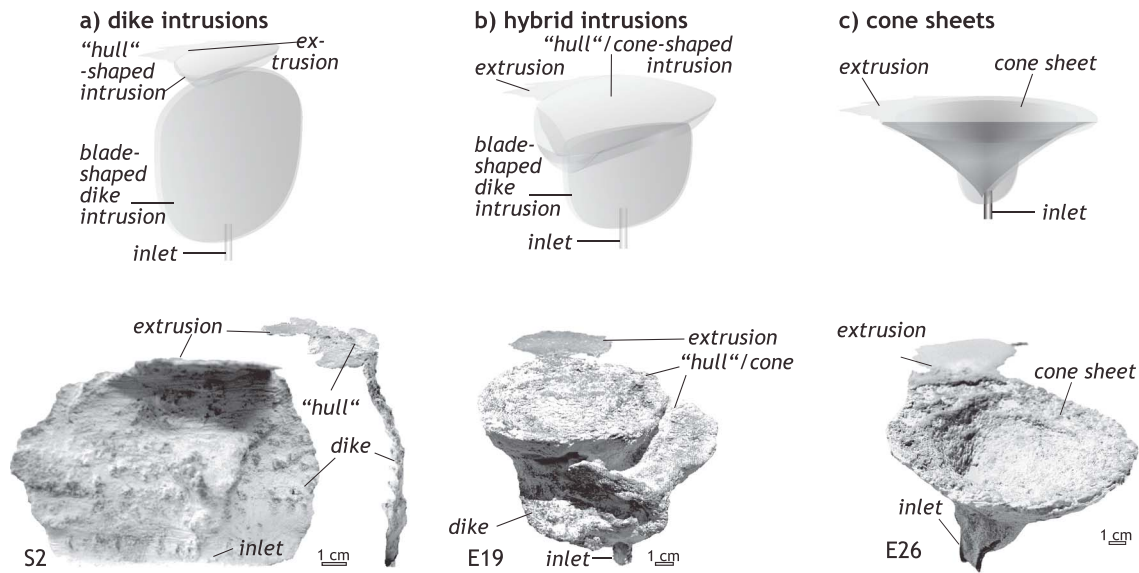
Figure 4. (a) Schematic drawing (top) and photograph (bottom) of a typical dike produced during the experiments and excavated from the host powder after solidification of the oil. The dike initiated from the inlet at the bottom and fed an elongated V-shaped, or “hull”-shaped, sheet intrusion to the very top. (b and c) Schematic drawings (top) and photographs (bottom) of typical excavated hybrid and cone sheet intrusions, respectively.
