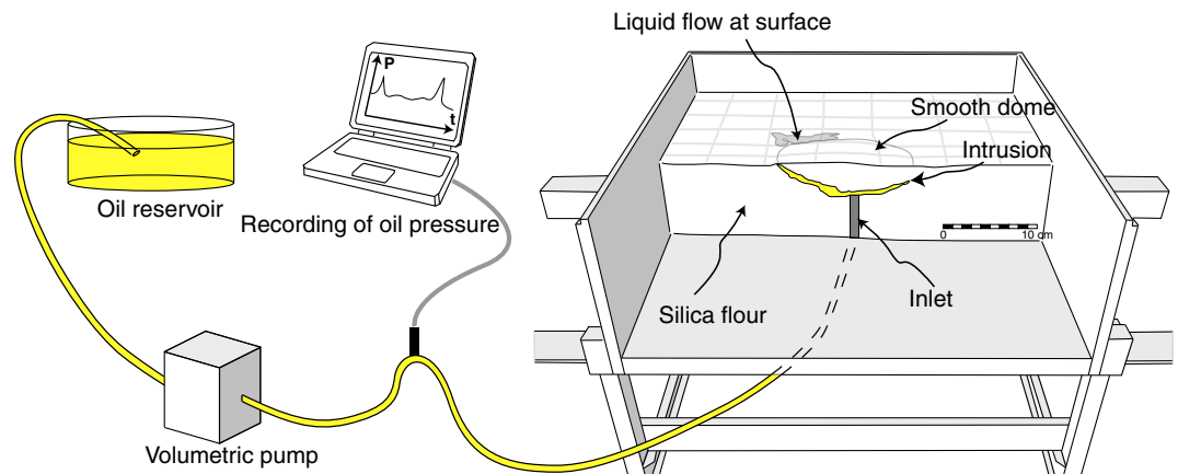
Figure 2. Drawing of the experimental apparatus used in this study.
