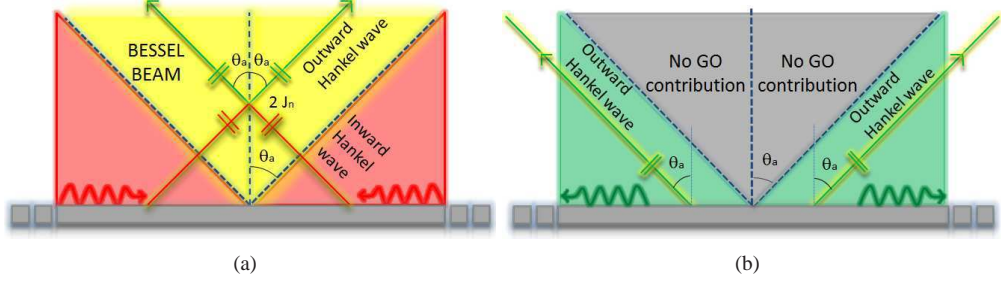
Fig. 2. Ray interpretation of the GO field for an infinite aperture. (a) Inward Hankel aperture distribution: the GO field comprises an inward Hankel beam ray (in red), present throughout the space, and an outward Hankel beam ray (in green) bounded inside the cone \theta < \theta_a ; the superposition of the two rays inside the cone (yellow area) creates a Bessel beam. (b) Outward Hankel aperture distribution: the GO field comprises only an outward Hankel beam ray (in green) bounded outside the cone \theta < \theta_a .
