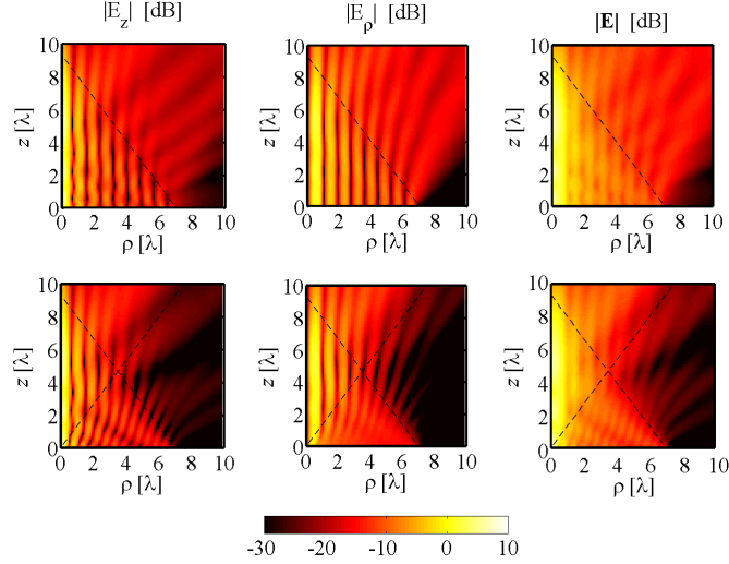
Fig. 4. Electric field radiated by an finite aperture with radius of a = 7\lambda . |E_z| (1 st column), |E_\rho| (2 nd column) and total electric field amplitude |\mathbf{E}| (3 rd column). Standard Bessel beam reference field (1 st row), and field radiated by an inward Hankel distribution (2 nd row). The axes are normalized with respect to the wavelength ( \lambda ) at the operating frequency f . The dashed line marks the GO boundaries.
