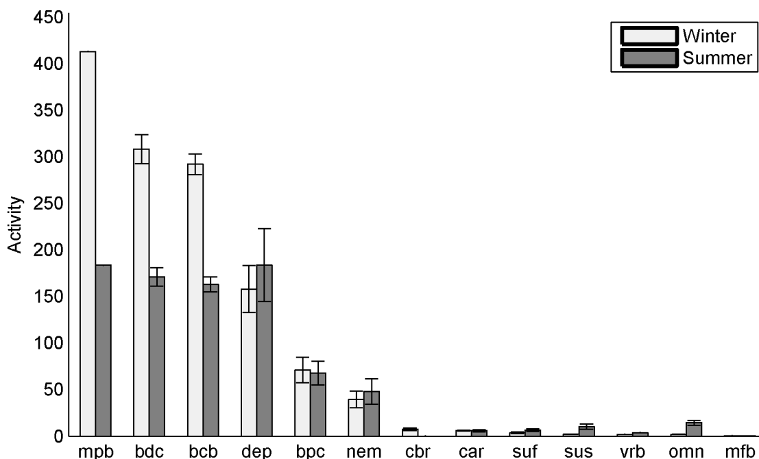
Figure 3. Compartment activities in \text{mgC}\cdot\text{m}^{-2}\cdot\text{LT}^{-1} for the two seasons. The error bars represent the standard deviation on the 500,000 simulations. See Table 1 for compartment abbreviations.
