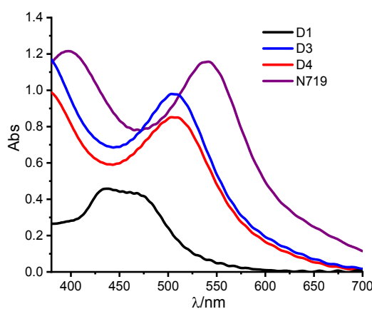
Figure 3. Absorption spectra of the complexes D1-D4 loaded on transparent TiO 2 films ( ca. 6 \mu\text{m} thick) sintered on FTO. Spectra were corrected against a background constituted by an otherwise identical undyed TiO 2 /FTO film.
