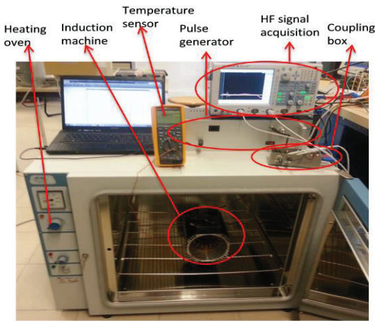
Fig. 4. Experimental bench.
