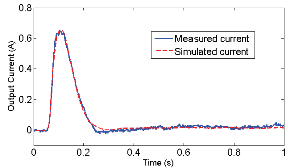
Fig. 6. Experimental measurement for a step excitation protocol
