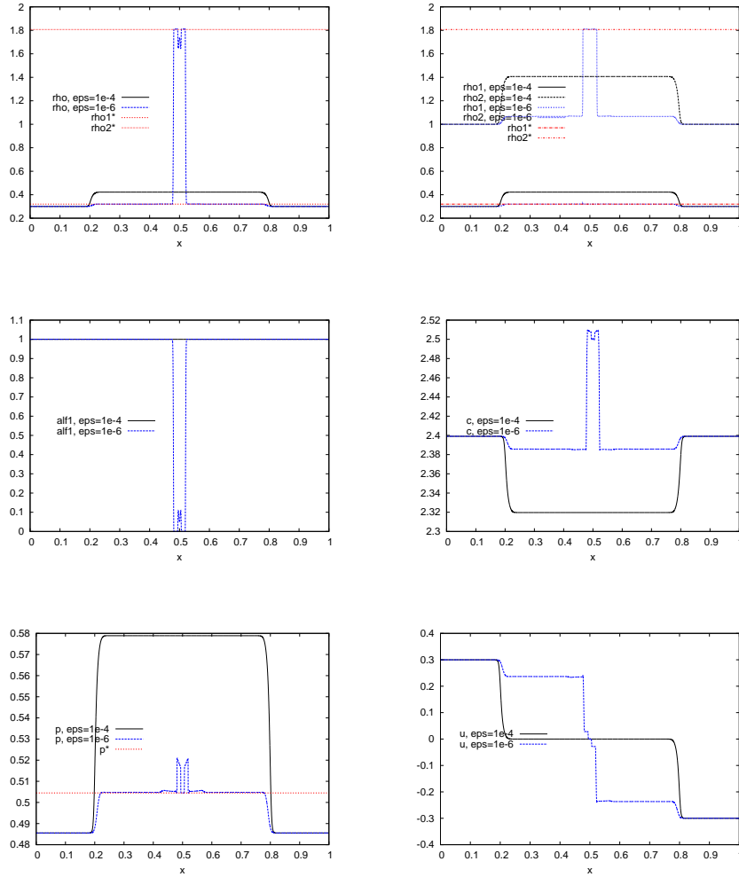
FIGURE 12. Nucleation by double shock. From top left to bottom right: density \rho , densities \rho_1 and \rho_2 , volume fraction \alpha_1 , speed of sound c , pressure p and velocity u .
