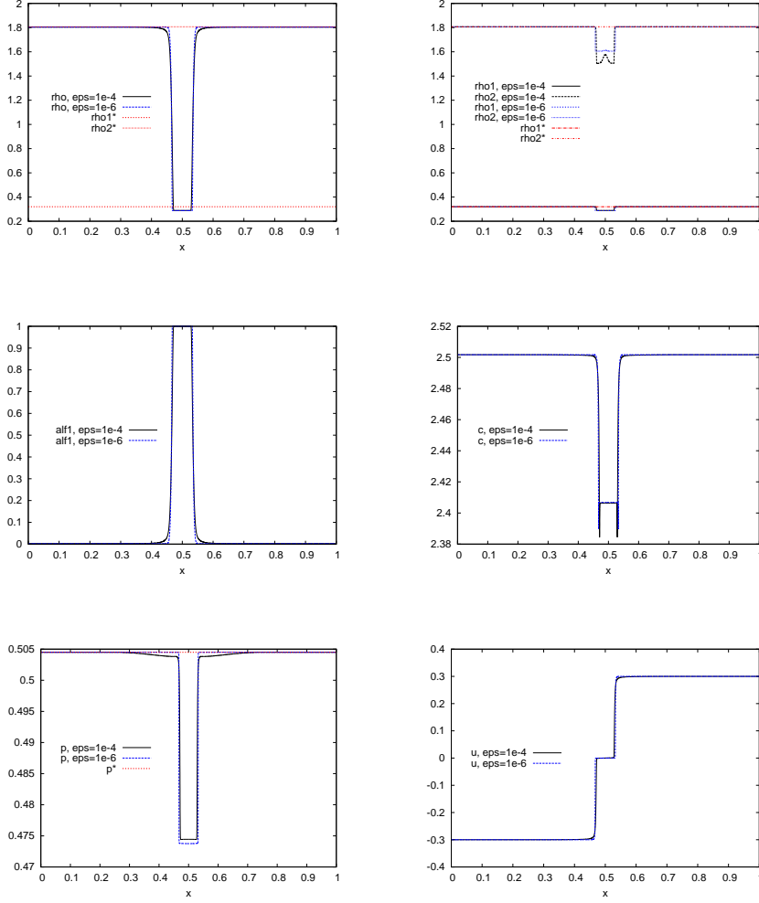
FIGURE 11. Cavitation by double rarefaction. From top left to bottom right: density \rho , densities \rho_{o1} and \rho_2 , volume fraction \alpha_1 , speed of sound c , pressure p and velocity u .
