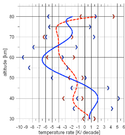
Figure 1. Temperature trends derived from the OHP lidar for winter (blue) and summer (red) periods with a multi-function linear regression.
