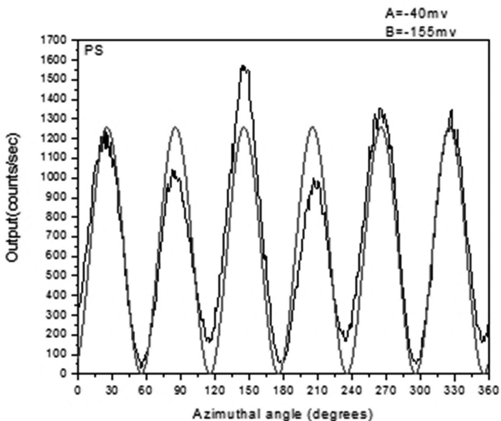
Figure 8. Second Harmonic intensity at PS polarization configuration in the function of rotation angle with the expectation curves using equation 10. (Made by author.)
