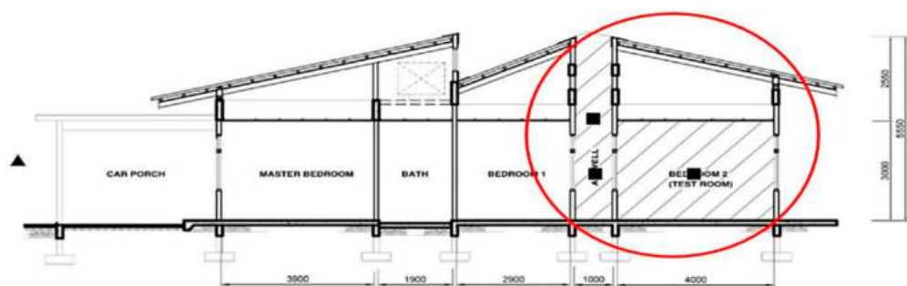
(b) The diagram shows the section drawing of the case study house. The hatched area and red circle indicates the position of case study room and air well. The core unit has been selected for the study instead of whole house since the performance of core unit gives precursors results to the extensive study in future.
