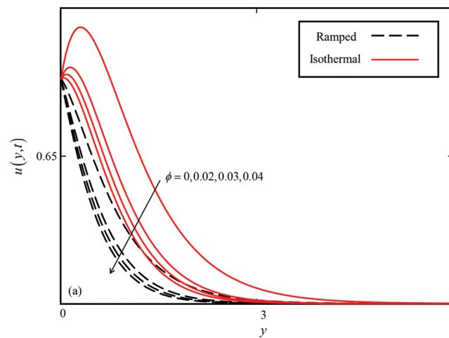
Figure 4: Consequence of \phi on u(y, t) when \alpha = 0.5 , \beta = 0.5 , M = 0.5 , Gr = 10 and \omega t = 0.15 for MWCNTs case
