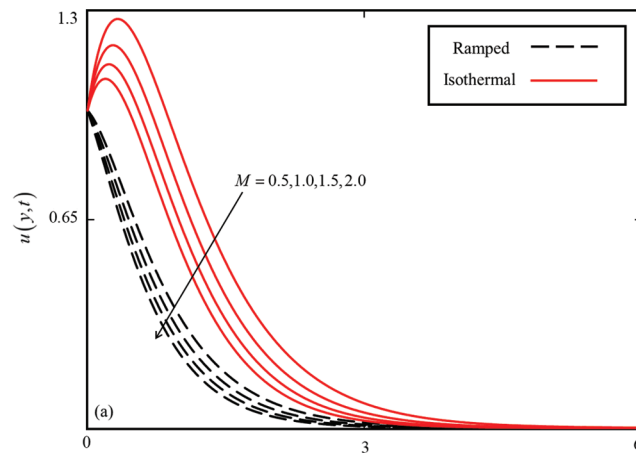
Figure 8: Consequence of M on u(y, t) when \alpha = 0.5 , \beta = 0.5 , \phi = 0.04 , Gr = 10 and \omega t = 0.15 for MWCNTs case
