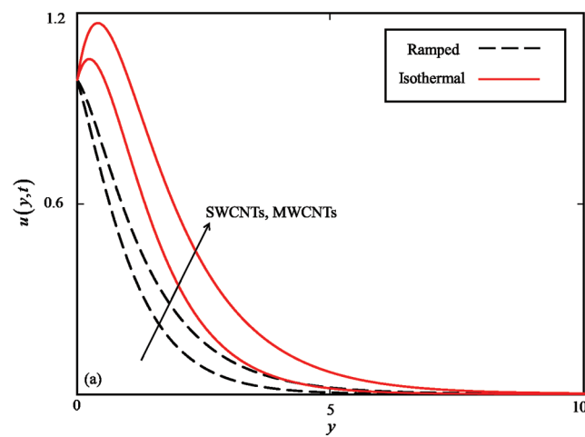
Figure 6: Comparison of u(y,t) for MWCNTs and SWCNTs when \alpha = 0.5 , \beta = 0.5 , \phi = 0.04 , M = 0.5 , Gr = 10 and \omega t = 0.15
