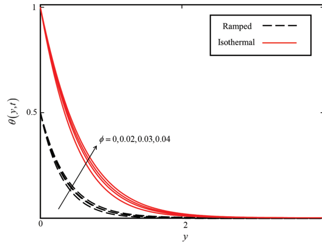
Figure 3: Consequence of \phi on \theta(y, t) when \alpha = 0.5 for MWCNTs case
