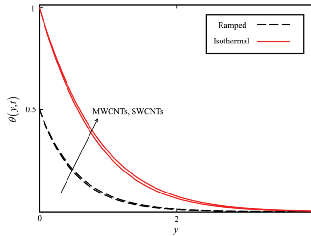
Figure 5: Comparison of \theta(y,t) for MWCNTs and SWCNTs when \alpha = 0.5 , and \phi = 0.04
