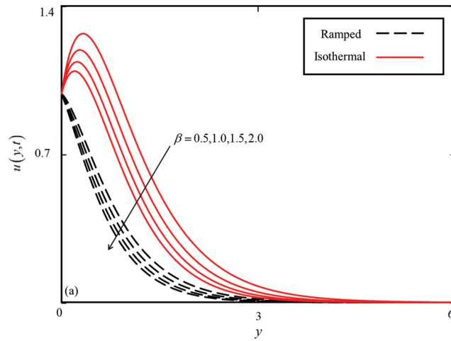
Figure 7: Consequence of \beta on u(y, t) when \alpha = 0.5 , \phi = 0.04 , M = 0.5 , Gr = 10 and \omega t = 0.15 for MWCNTs case
