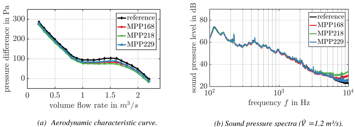
Figure 7: Influence of MPP absorbers on aerodynamic properties and sound pressure level spectrum.
