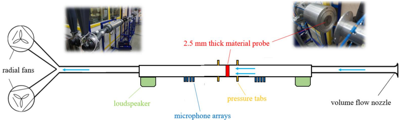
Figure 4: Illustration of the two-port test rig. The test rig can be excited with acoustic sound waves using two loudspeakers and flow can be generated using radial fans. The material samples are mounted in the center of the test rig.
