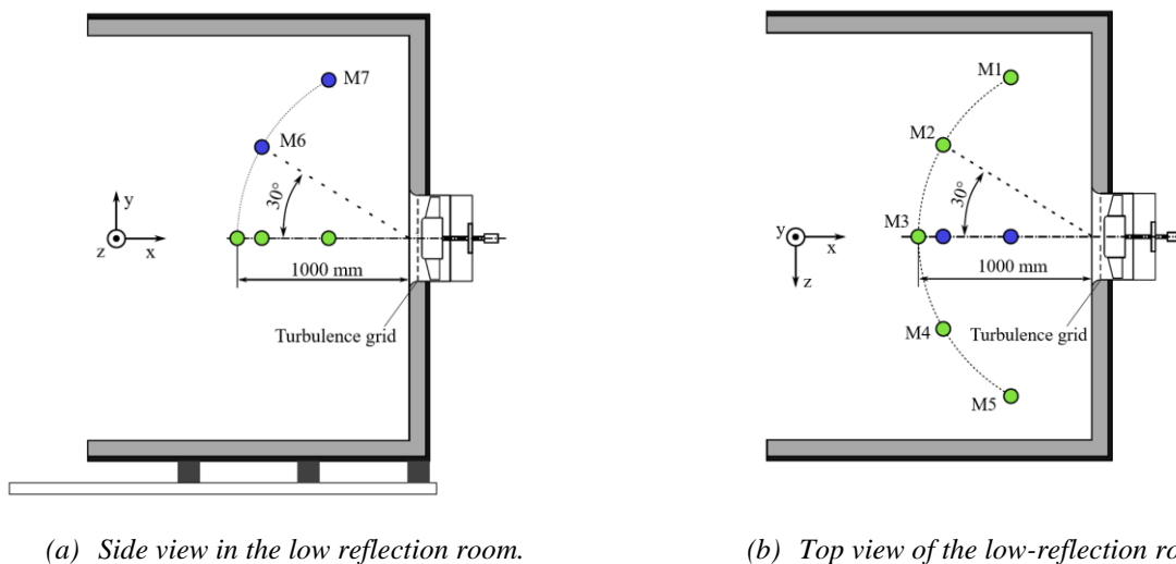
Figure 5: Schematic representation of the test setup for determining the aeroacoustics properties. Five microphones (M1-M5) are placed on a horizontal semicircle and two microphones (M6-M7) are placed on a vertical semicircle.
