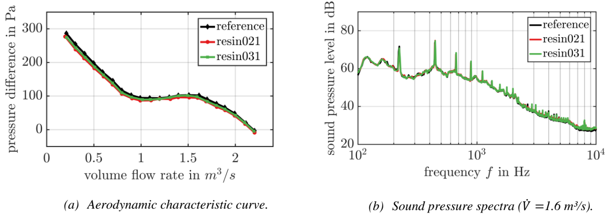
Figure 8: Influence of micro-porous resin on aerodynamic properties and sound pressure level spectrum.
