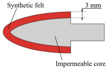
(a) Leading edge with felt lining.
