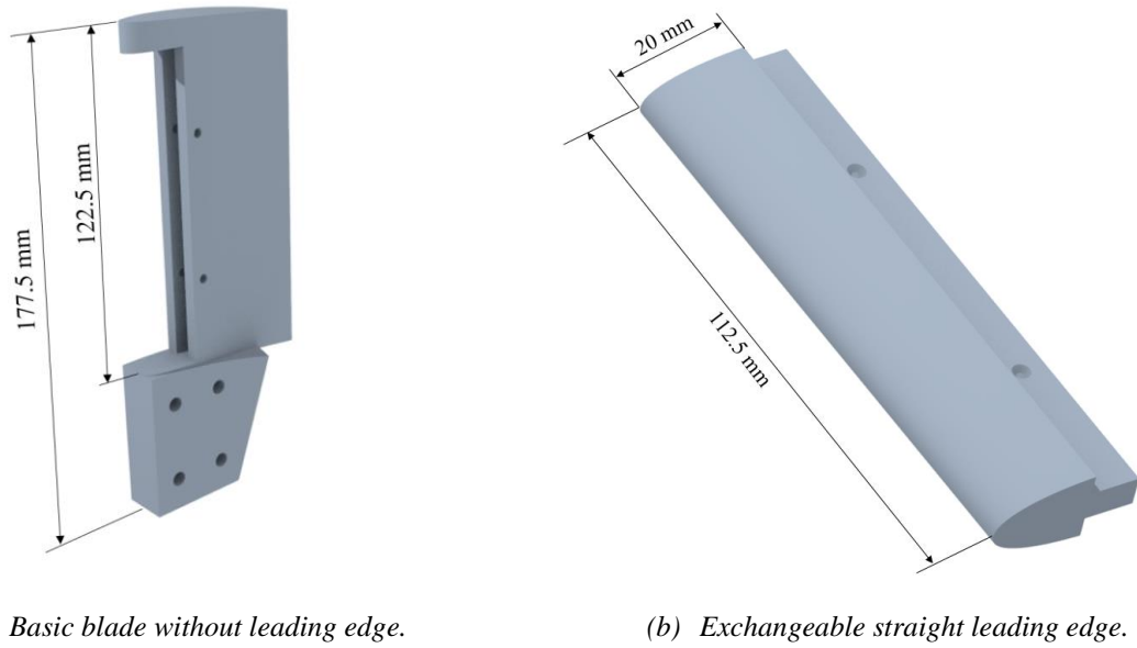
Figure 1: Illustration of the basic blade and a replaceable leading edge. The two components can be connected via a groove and two flat-head screws. In order to provide additional radial securing, the tip area of the blade is designed to be solid.
