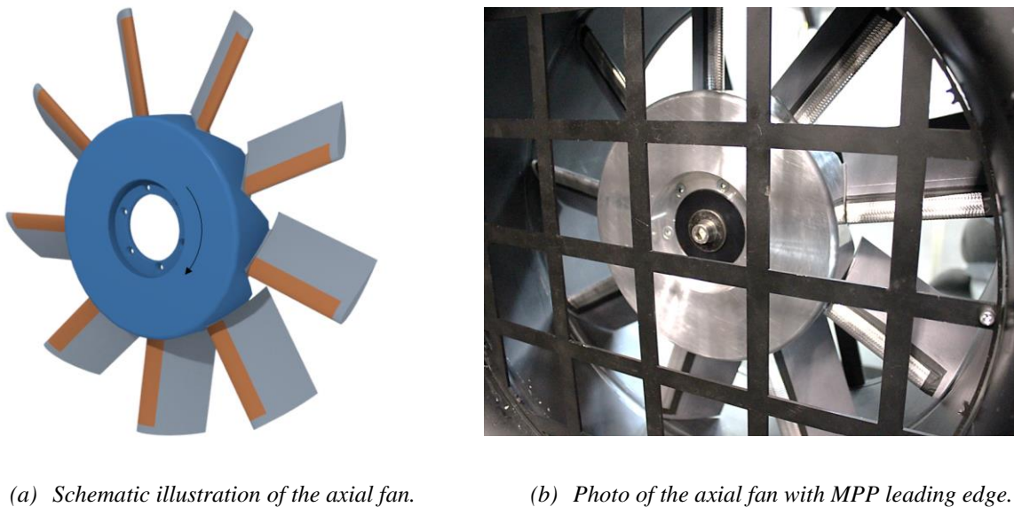
Figure 2: Schematic representation of the axial fan (a) with NACA 0018 profiles as blades. The replaceable leading edges are shown in orange. Photo of the installed axial ventilator with turbulence grid and MPP leading edge (b).
