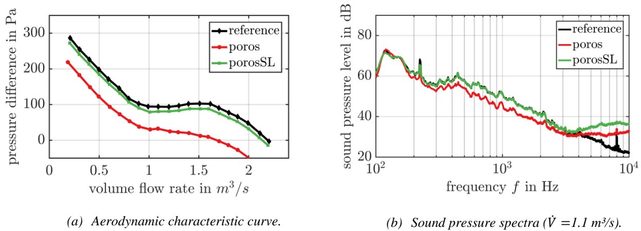
Figure 9: Influence of a structured porosity and separation layer on the aerodynamic and acoustic properties.
