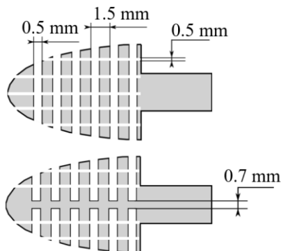
(g) Structured porosities with and without separation layer.
