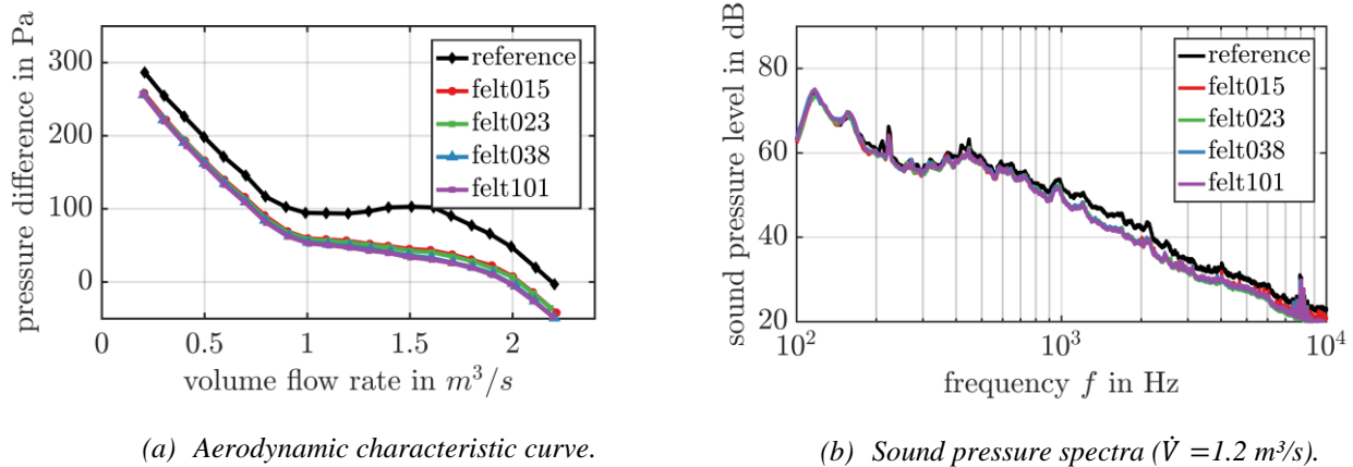
Figure 6: Influence of felts on aerodynamic properties and sound pressure level spectrum.
