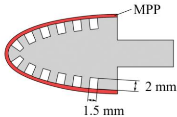
(c) Leading edge with MPP surface.
