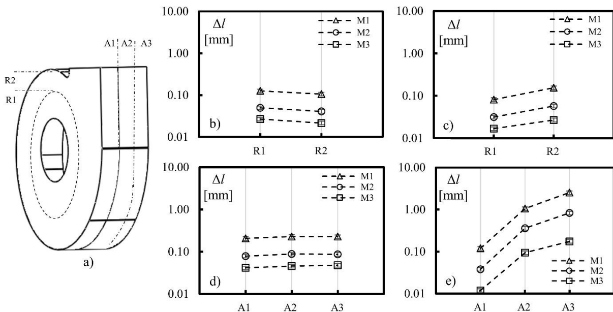
Figure 7: Volute wear: a) coordinates of the patches on volute, and material loss b) on the front side, c) backside, d) lateral side, and e) cut-off.
