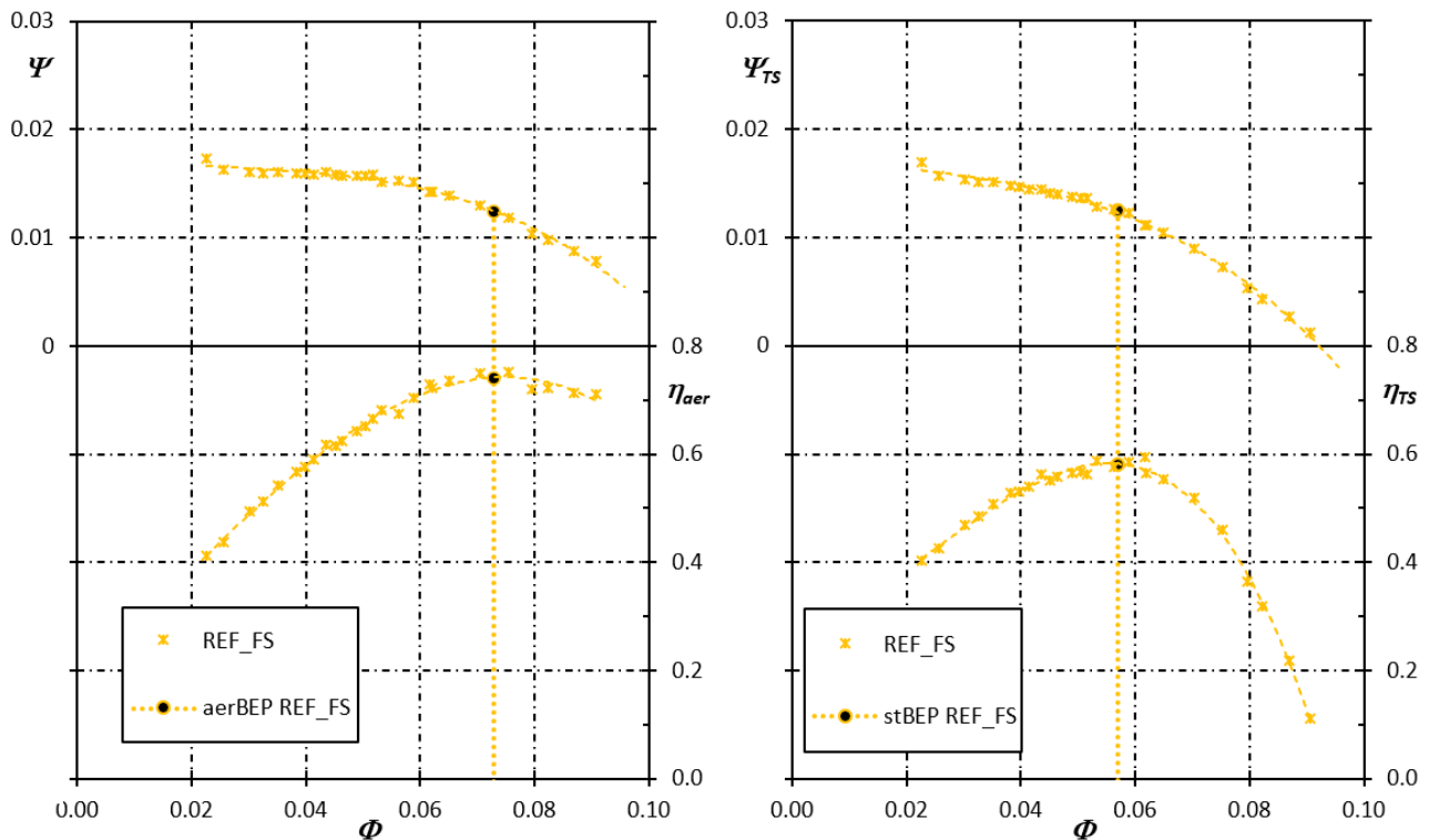
Figure 1: full scale data of the REF_FS fan (orange asterisk markers, adapted from [1]). Filled circles mark the best efficiency operation.
