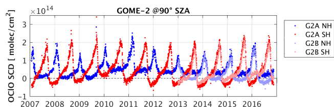
Figure 2. Daily GOME-2 OCIO SCD time series for SZAs of 90 \pm 1^\circ .
