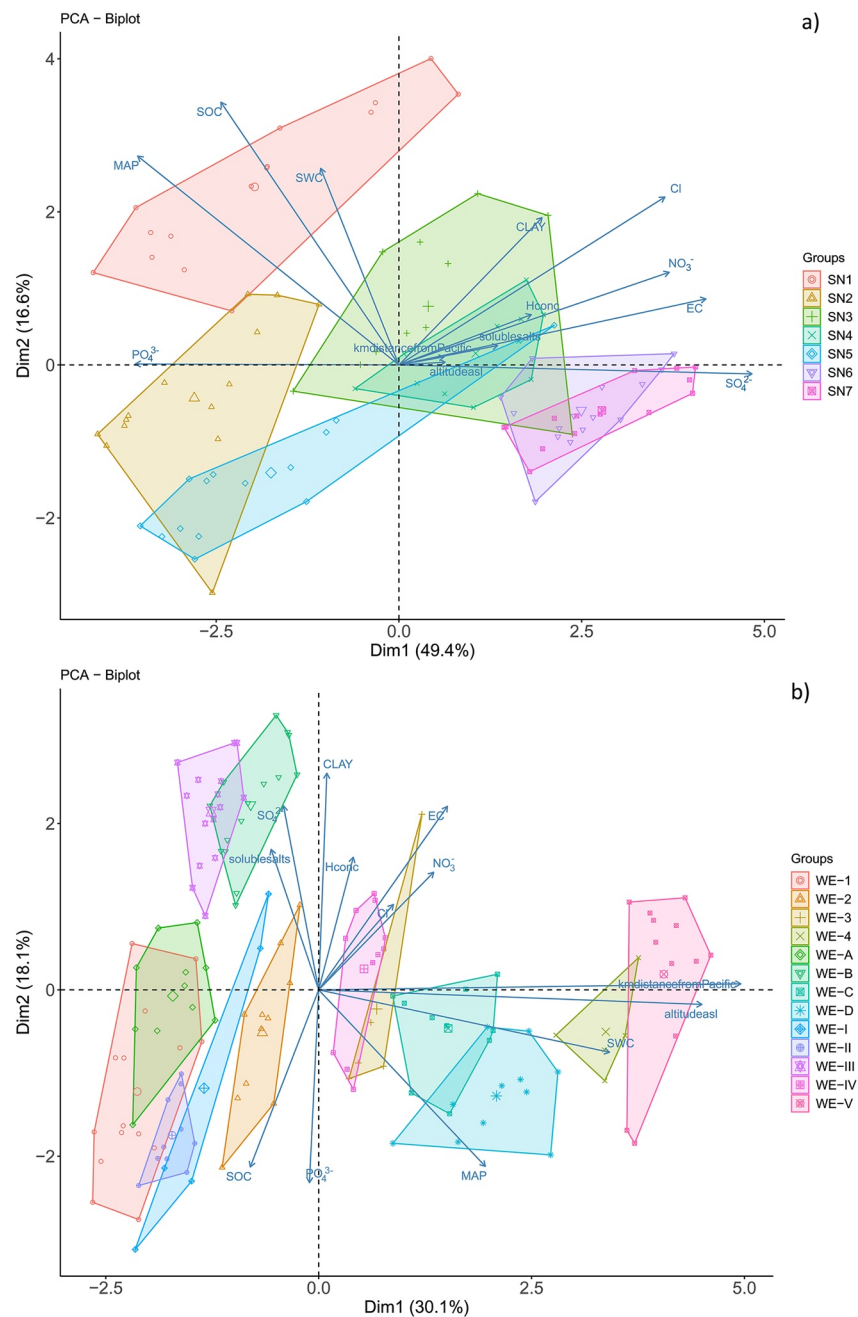
Figure 4. (a) Principal Component Analysis (PCA) for the South-North gradient. Salts, pH, and CLAY (with the exception of \text{PO}_4^{3-} ) correlate positively with each other, while SOC, SWC, and MAP is correlated positively with each other. The length of the variable's arrows indicate the grade of impact on the sites. A clear shift from the arid plots SN-1 and SN-2 toward the hyper-arid plots SN-6 and SN-7 indicates a gradual change of properties along the gradient and significant differences among the climatic regimes. (b) The PCA along the three West-East transects shows that altitude asl and distance from the Pacific have the strongest impact on the data. They are positively correlated with each other, with SWC and with MAP but uncorrelated with SOC which is in contrast to the SN gradient, where the occurrence of SOC is positively correlated with precipitation.
