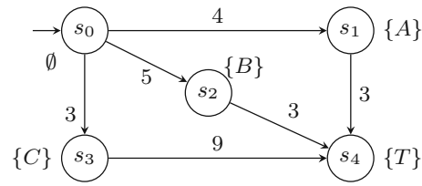
Fig. 4 Example CTMC
