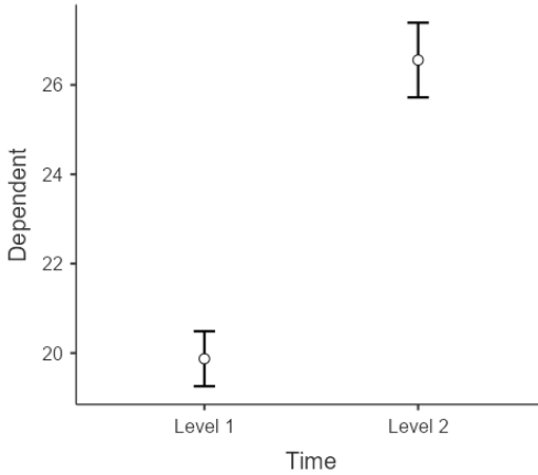
Estimated Marginal Means - Time
