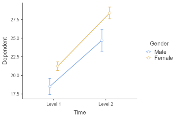
Estimated Marginal Means - Time * Gender
