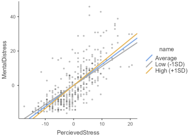
Simple Slope Plot
