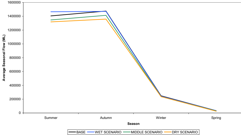
Currareva for Base Scenario and Three Climate Change Scenarios
