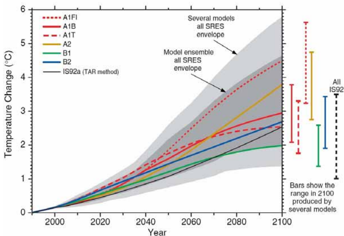
Figure 2. Global mean temperature projections for the six illustrative SRES scenarios using a simple climate model tuned to a number of complex models with a range of climate sensitivities. Also for comparison, following the same method, results are shown for IS92a. The darker shading represents the envelope of the full set of thirty-five SRES scenarios using the average of the models results. The lighter shading is the envelope based on all seven model projections (from IPCC, 2001).
