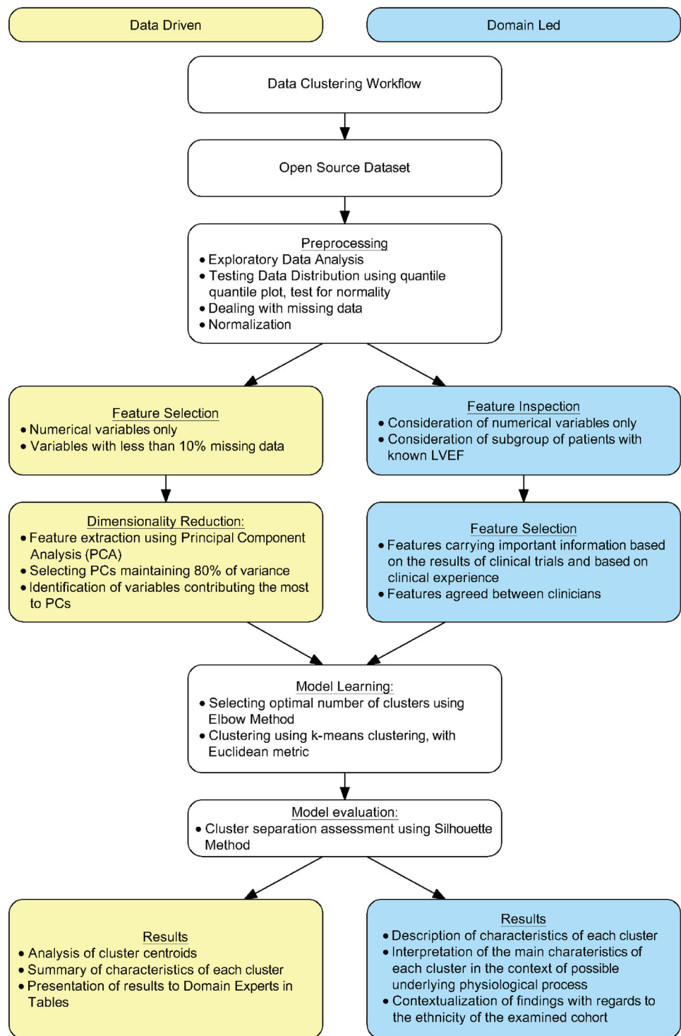
Fig. 7 This figure shows learning processes used during clustering experiment. The branches on the left (shown in yellow) present stages unique to the data-driven approach, whereas the branches on the right (shown in blue) present stages unique to the domain-led approach
