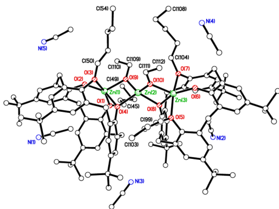
Fig. 4 Molecular structure of [\text{Zn}_3(\text{OEt})_2(\text{L}(\text{O})_2(\text{On-pentyl})_2)_2] \cdot 4.5\text{MeCN} (4·4.5MeCN). H atoms and minor disorder components omitted for clarity. Selected bond lengths (Å) and angles (°): Zn(1)–O(1) 2.221(2), Zn(1)–O(2) 1.853(3), Zn(1)–O(3) 2.437(2), Zn(1)–O(4) 1.987(2), Zn(1)–O(9) 1.962(3), Zn(2)–O(4) 1.982(2), Zn(2)–O(8) 1.983(2), Zn(2)–O(9) 1.942(3), Zn(2)–O(10) 1.937(3); Zn(1)–O(4)–Zn(2) 97.14(10), Zn(1)–O(9)–Zn(2) 99.32(12), Zn(2)–O(10)–Zn(3) 99.08(11).
