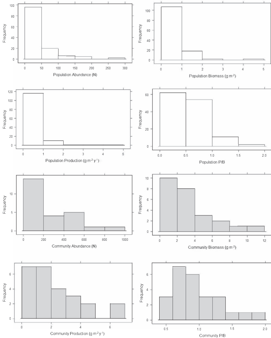
FIGURE 4 Relative frequency histograms of individual fish population abundance ( N ), production ( \text{g m}^{-2} \text{y}^{-1} ), biomass ( \text{g m}^{-2} ) and annual P/B, and fish community abundance, production, biomass and annual P/B for the 25 sampled streams across the Appalachians
