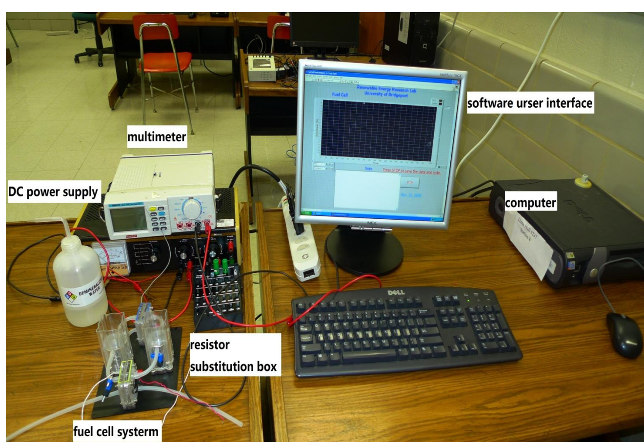
Figure 4. Setup for the VI measurement of a fuel cell
