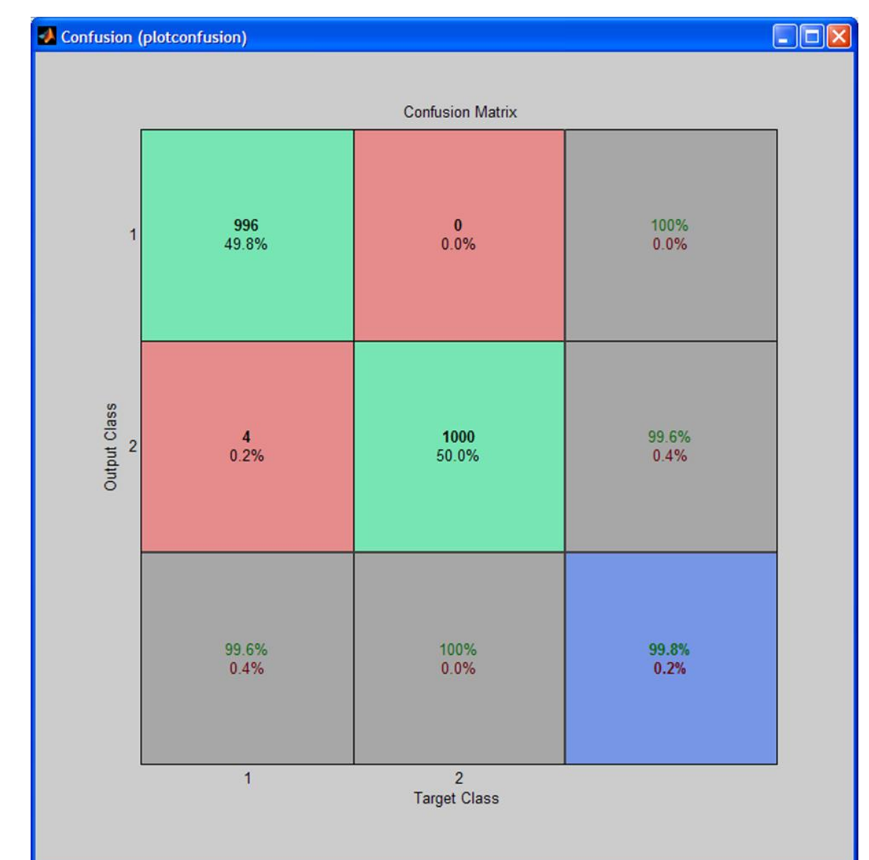
Classification confusion matrix for 1000 wav files
