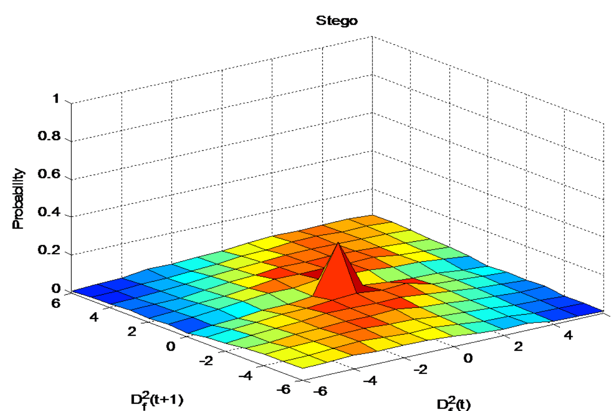
Markov transition probability of the second order derivative (Stego wav)
